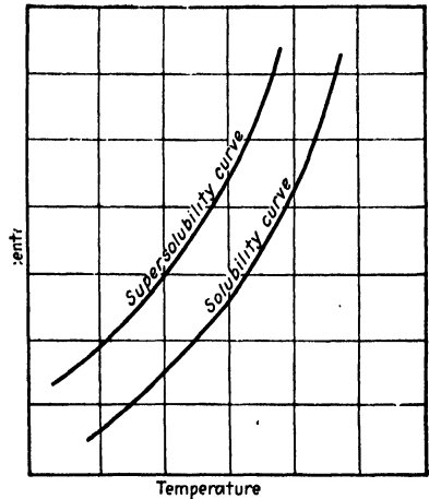
FIG. 5.—Temperature-concentration diagram of a typical solution.
